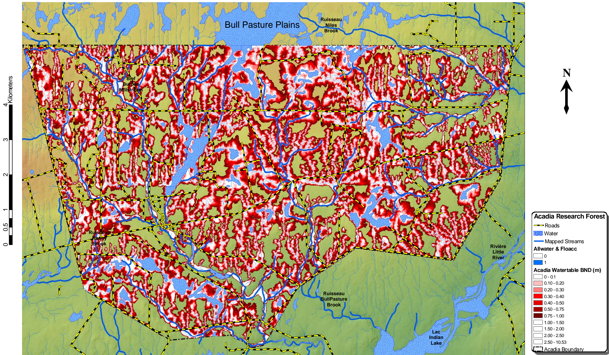
Acadia Research Forest – Depth-to-Water Table Map: 5 m resolution, varying from < 10 cm (white) to 100 cm (red)
